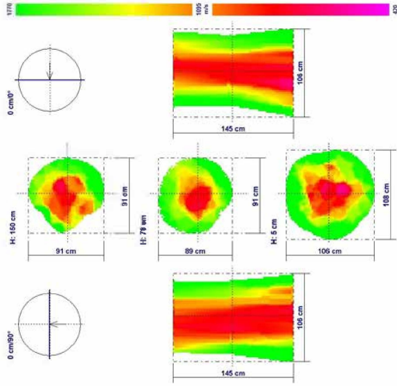
Figure 6. This tree has stood close to a subtropical coastal shore line for more than 100 years. As shown by the sonic tomogram, the stem has been severely damaged and hollow for decades but has survived dozens of hurricanes while young intact trees in the same area broke. This illustrates that the older trees are the higher their basic safety and the more decay the can tolerate without being significantly more susceptible to breakage.
