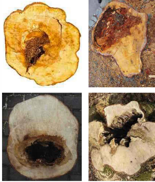
Figure 5. Examples from typical mature urban trees to be inspected in terms of safety: the cross-sections are commonly not circular and the defects are mostly located off-center. Such cross-sections provide many different radius values and many different shell-wall thicknesses (t), often ranging from zero (t=0) to fully wooded (t=Radius). Consequently, there is no typical or average t/R that could be quickly determined at the tree. Furthermore, minimum, maximum, or average t/R values do not represent the load-carrying capacity of such cross-sections. In consequence, the One-Third Rule simply does not apply to these kind of trees.
